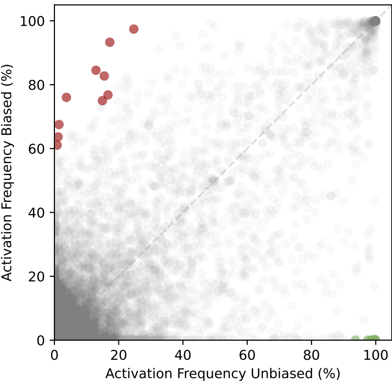
Activation Frequencies of SAE Latents: Race_1
